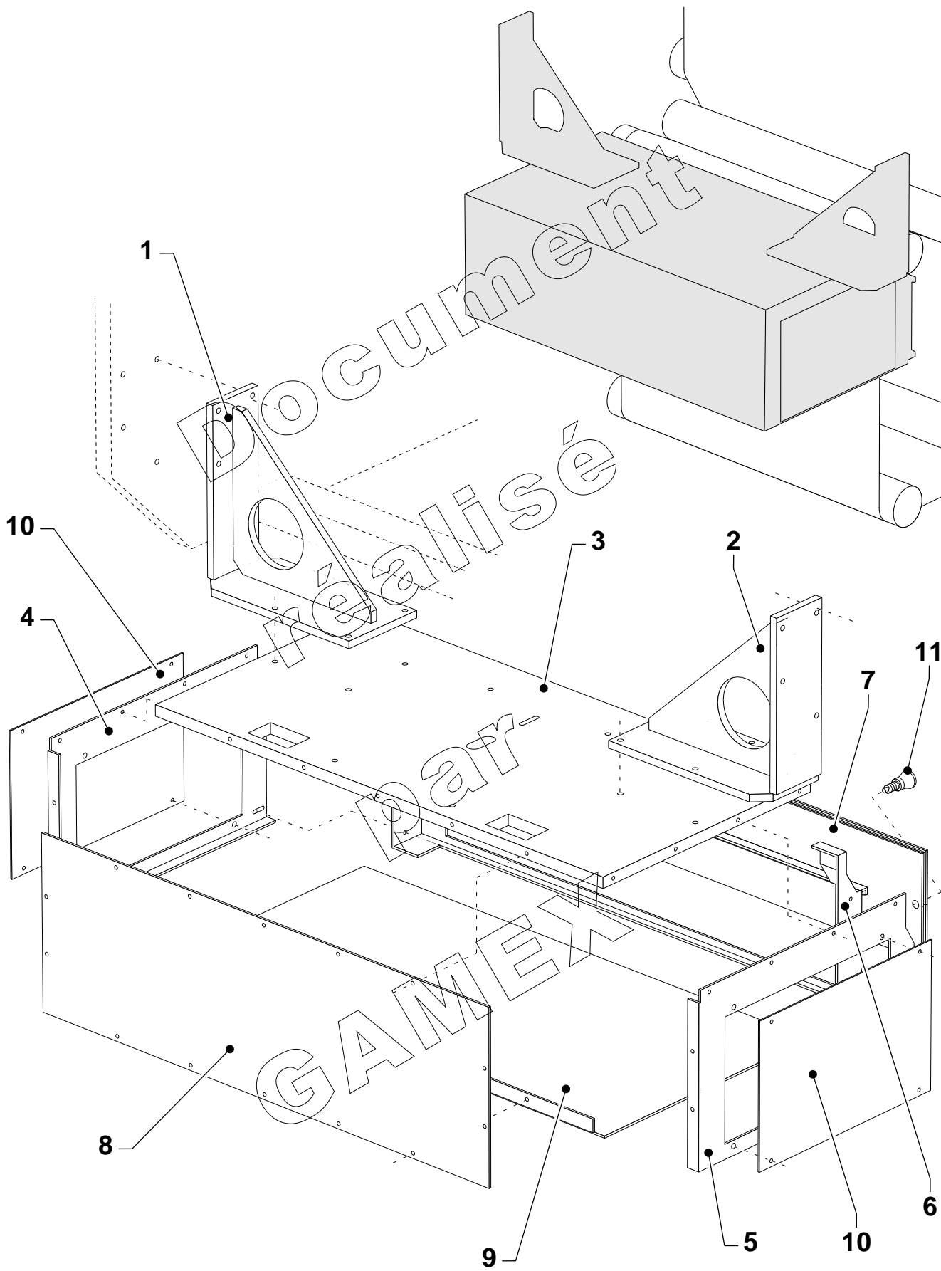
ENSEMBLE CAISSON (planche 5-3)
